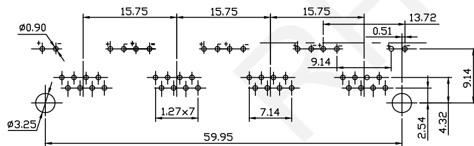
PCB Layout
